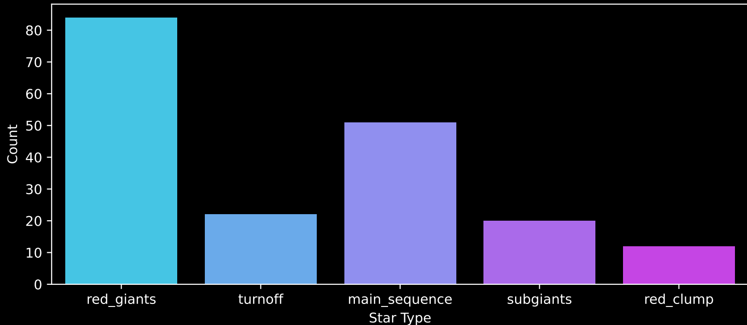
APOGEE DR17 Field: [K2_C7_016-13_btx] Count plot of Star Type
