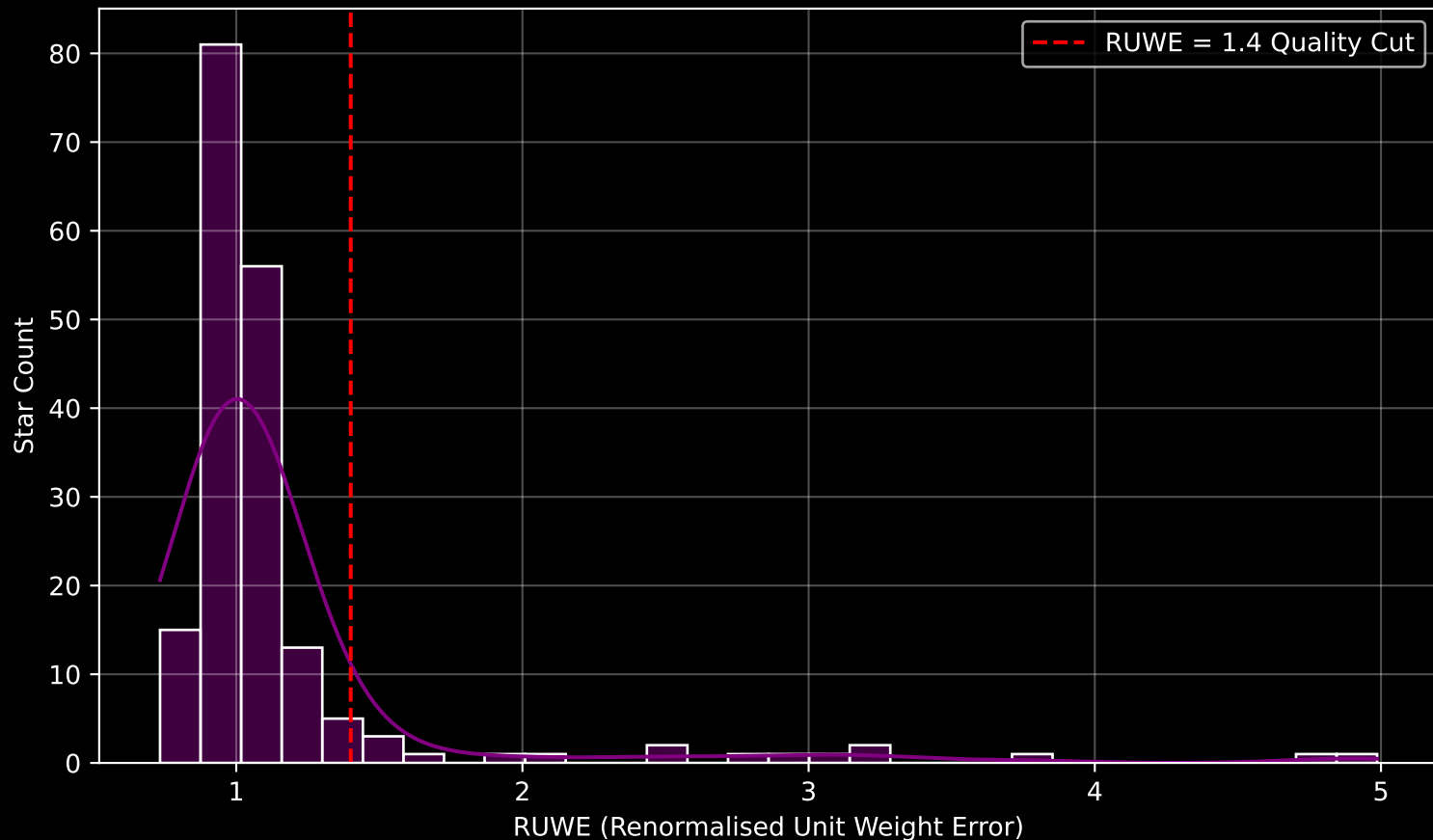
GAPOGEE DR17 Field [K2_C7_016-13_btx] RUWE Distribution (n= 186)
