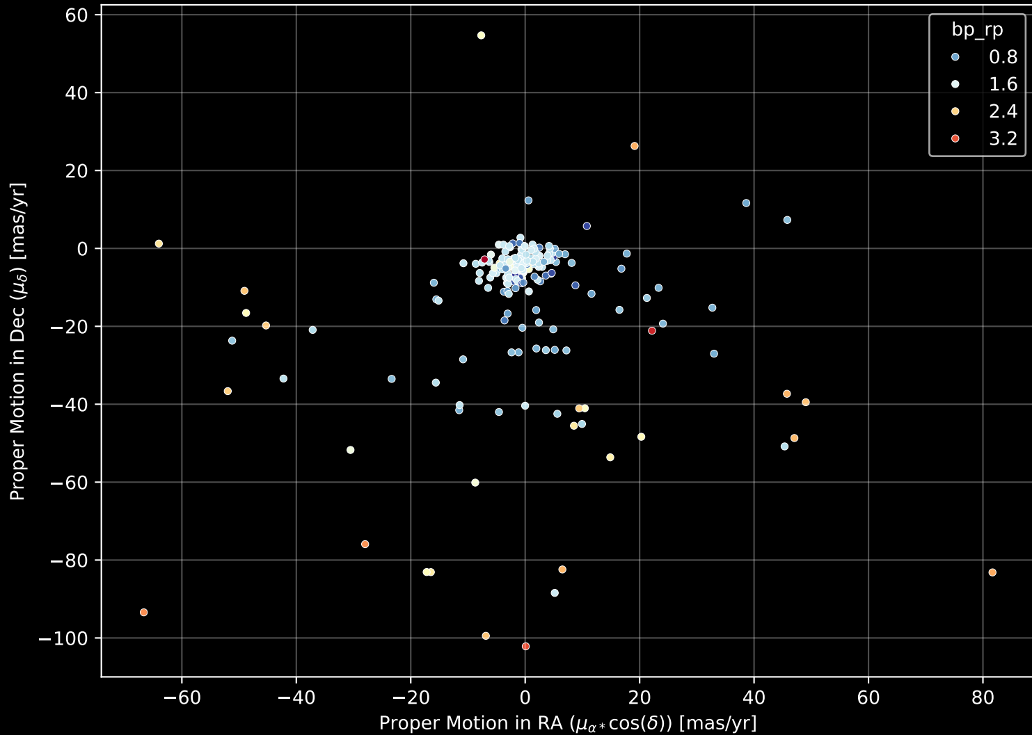
APOGEE DR17 Field: [K2_C7_016-13_btx] Proper Motion Diagram (n= 189)
