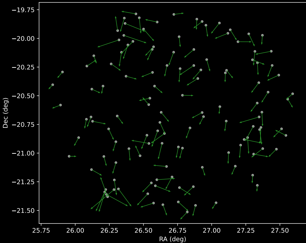
APOGEE DR17 Cluster 4 Proper Motion Vectors (n=126)
