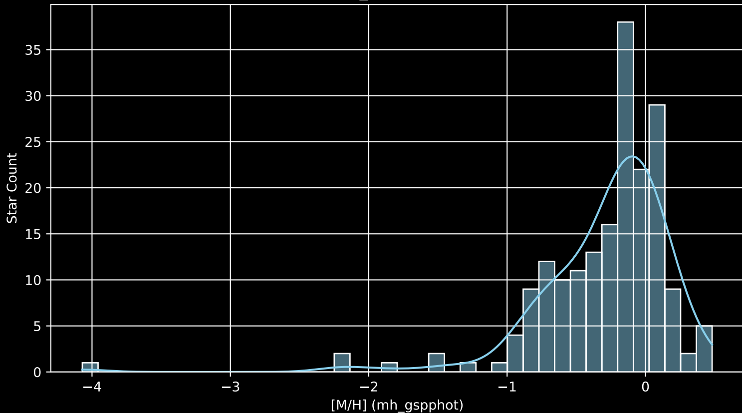
APOGEE DR17 Field: [K2_C7_016-13_btx [M/H] (mh_gspphot) (n= 188)
