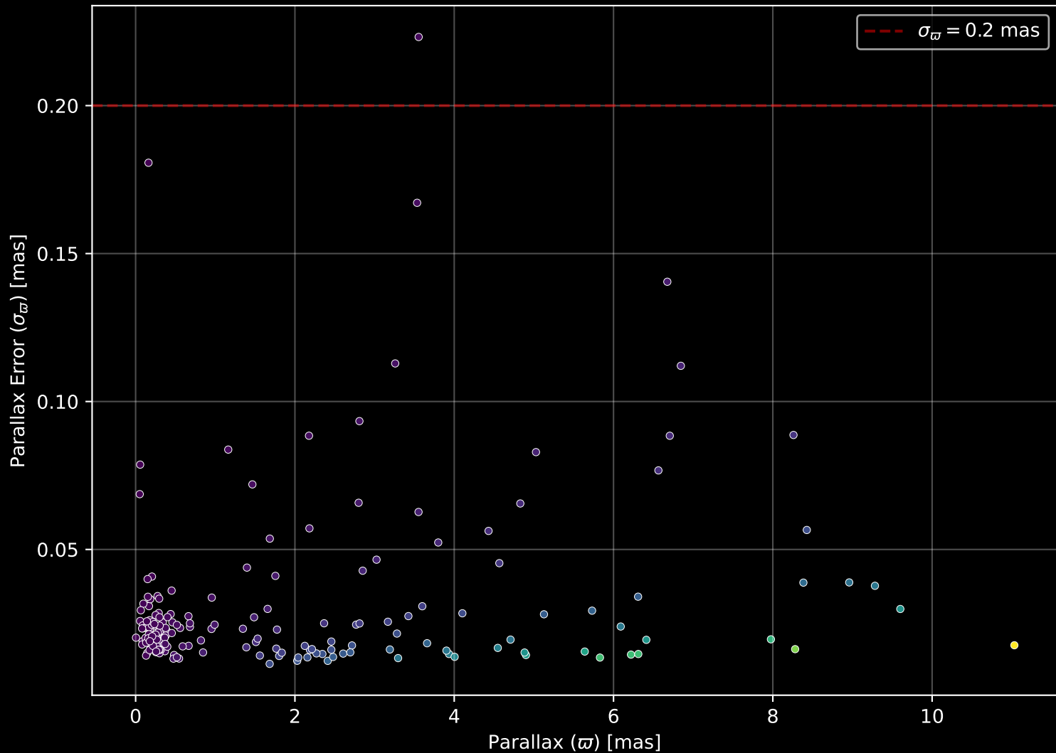
APOGEE DR17 Field: [K2_C7_016-13_btx] Parallax Quality (n= 189)
