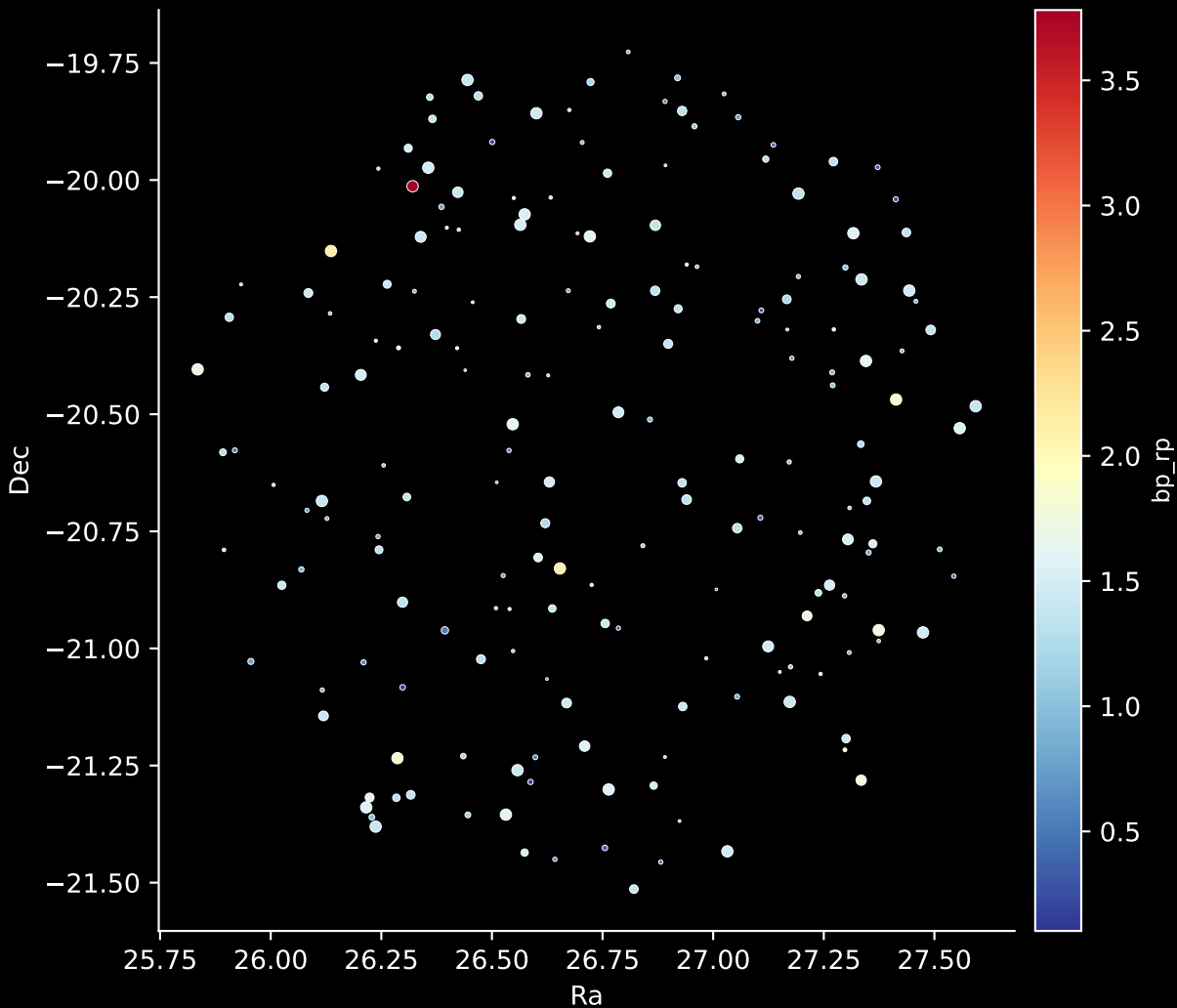
APOGEE DR17 Field: [K2_C7_016-13_btx] Stars: 189
